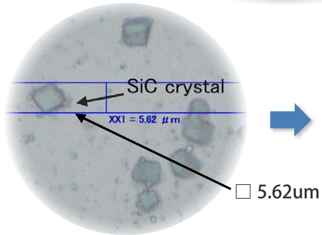
No applied vibration
