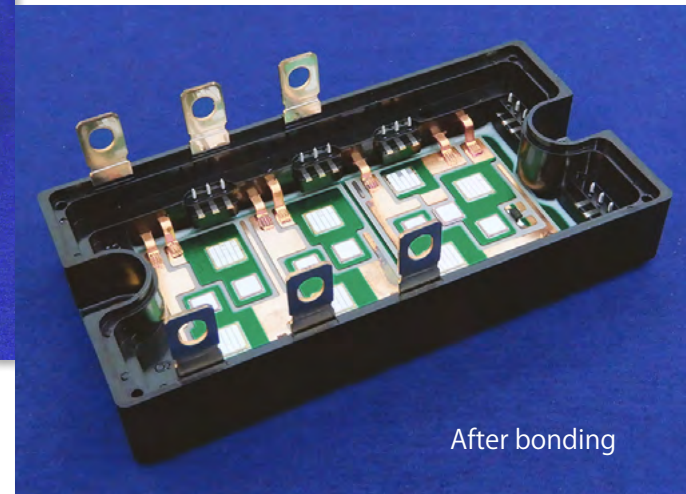
Power module for robot control
