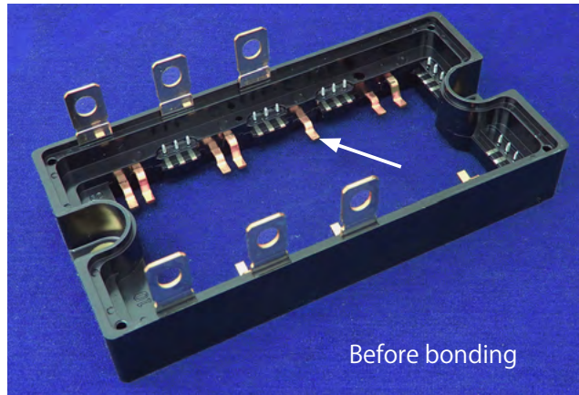
Power module for robot control
