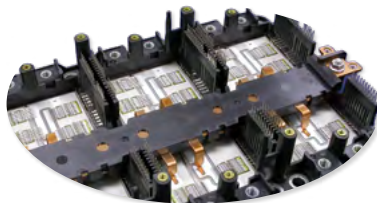
High power type power module for automobiles
