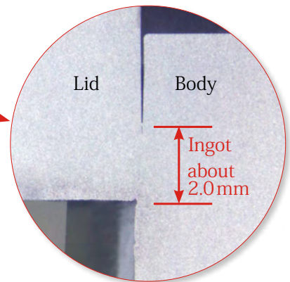
[Cross section of bonding part]
