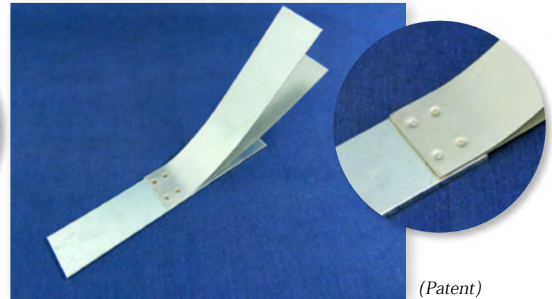
② Upper 2 plates SUS304 (@t=0.5mm) Bottom 1 plate Galvanized steel (t=2.3mm)
