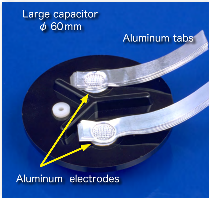
Bonding of Aluminum tabs to Aluminum electrodes directly
