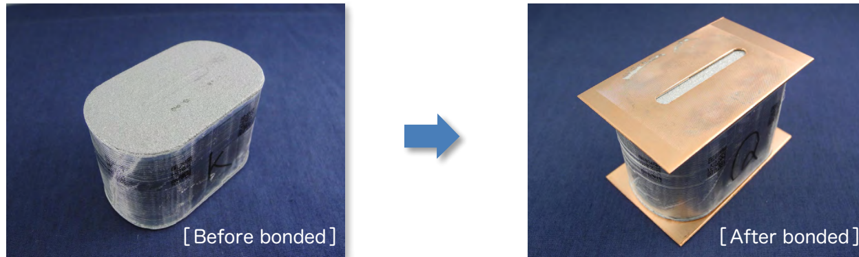
[ Double sided bonding of extra-large film capacitor between Zinc layer and Copper electrode ]
