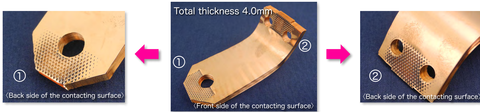
[ Multi-bonding of 40-layered Copper sheets 0.1mm thickness ]
