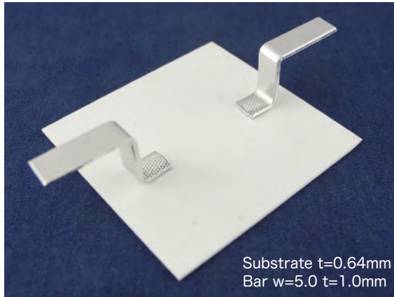
★ [Alumina substrate & Aluminum bus bars]
