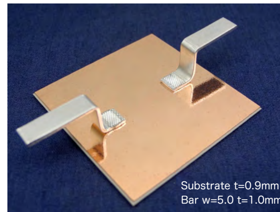
★ [AMC substrate & Aluminum bus bars]
