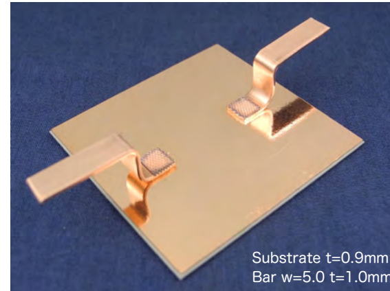
★ [AMC substrate & Copper bus bars]
