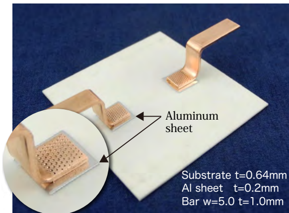
★ [Alumina substrate & Copper bus bars] Bonding by sandwiching Aluminum sheet
